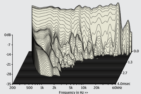
ABOVE: Cabinet resonances are well controlled while all cone modes are held to an impressively low level
